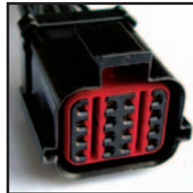
WPT326 3U2Z-14S411-JVA
