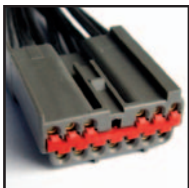
WPT612 3U2Z-14S411-YPA
