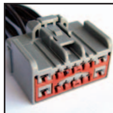
WPT741 3U2Z-14S411-BJAA
