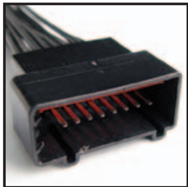
WPT650 3U2Z-14S411-LFA
